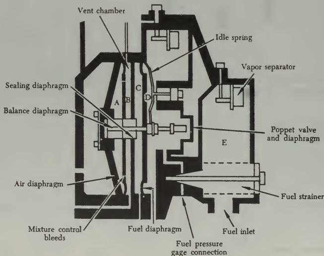
FIGURE 3-18. Regulator unit.
